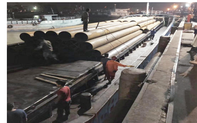
广西平南三桥 Pingnan third bridge, Guangxi. 2000 tons
